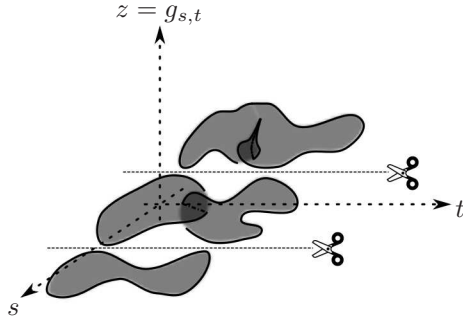
Figure 21: After the first cuts, along constant s slices. Note that components are still not embedded, due to the bad swallowtail.
