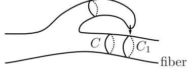
Figure 27: A 1-handle sliding over a 2-handle in a 2-parameter family.
