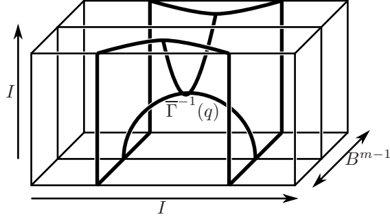
Figure 37: The model for \bar{\Gamma}^{-1}(q) in the statement of Lemma 6.2.
