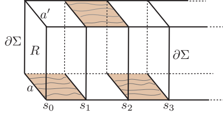
Figure 41: The zig-zag argument for Morse 2-functions
