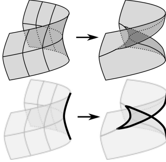
Figure 33: Bending a forward handle to a backward handle. The point is to see that the only change to the projection to the horizontal axis in this homotopy is that the critical point moves a little to the left, but that when we look at the map to 2 dimensions, i.e. projection to the page exactly as in this figure, the fold at the critical point changes from opening to the right to opening to the left. This figure is in fact nothing more than the standard homotopy that introduces a swallowtail.
